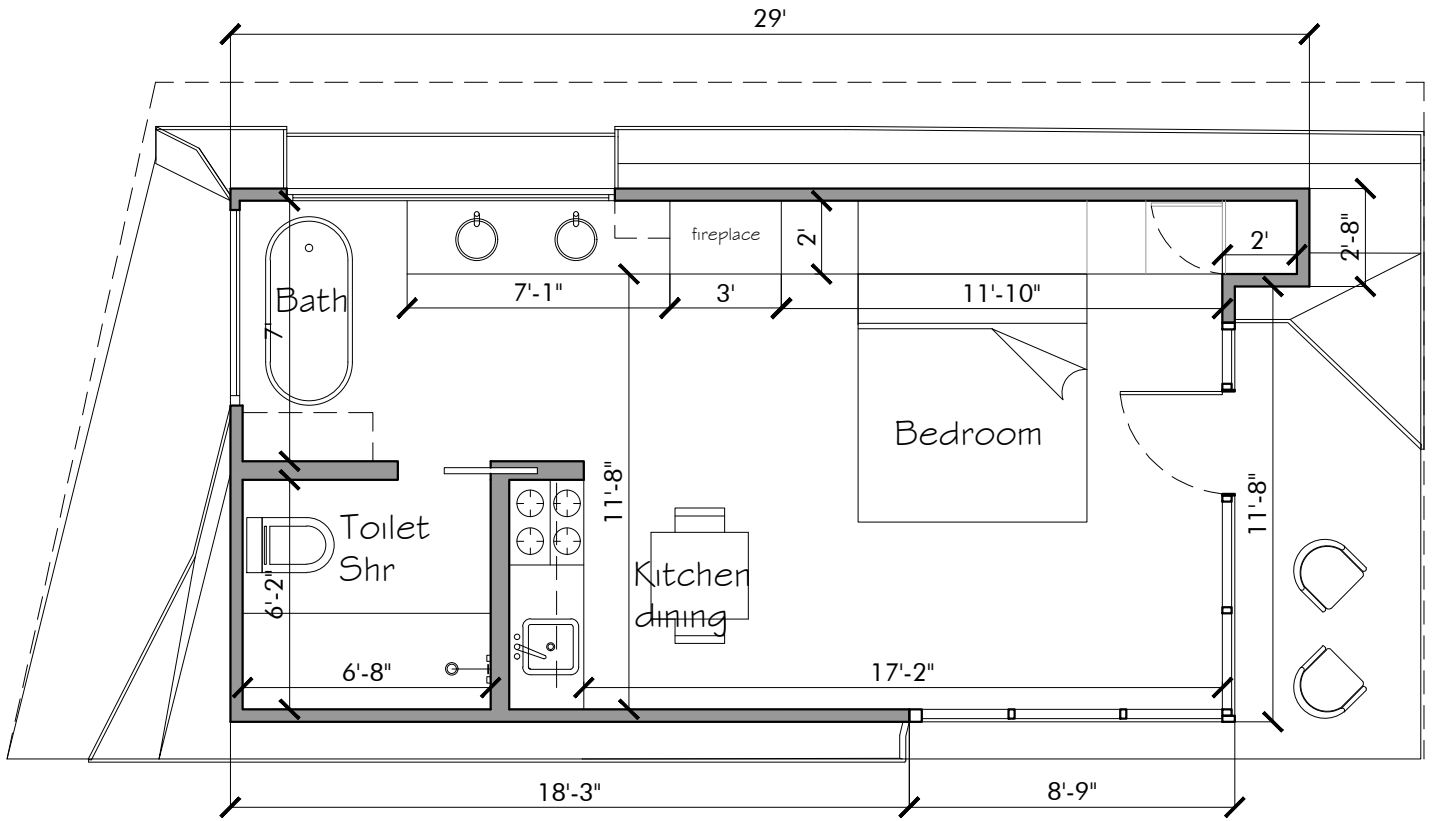
Floor Plan 400sqf
